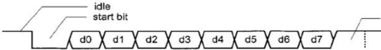
Figure 2.2: Transmission of a byte.
