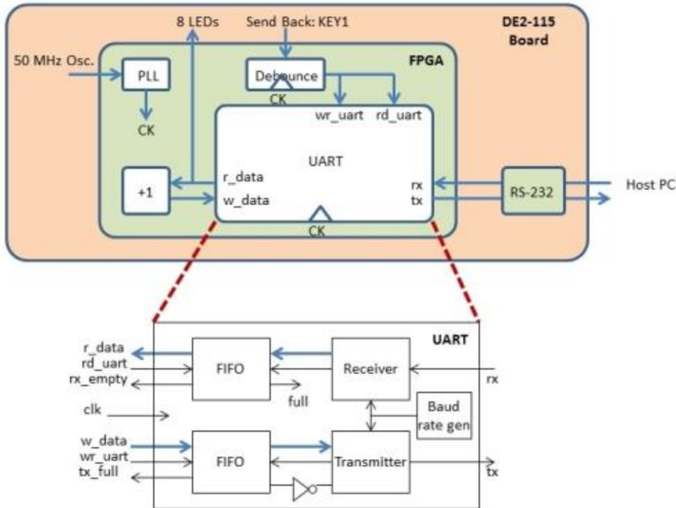
Figure 3.1: Block diagram of design that uses VHDL UART controller to connect FPGA of DE2-115 board to host PC.
